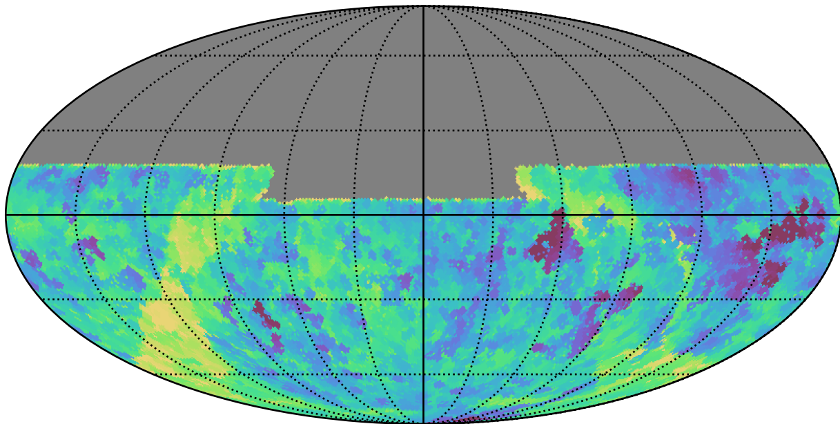
baseline_v2.0_10yrs All sky y band: Min fiveSigmaDepth
