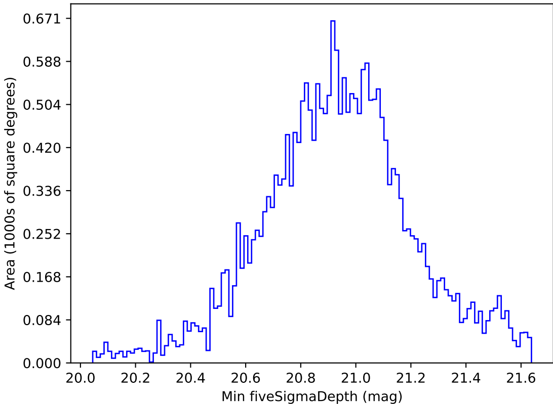
baseline_v2.0_10yrs All sky y band: Min fiveSigmaDepth
