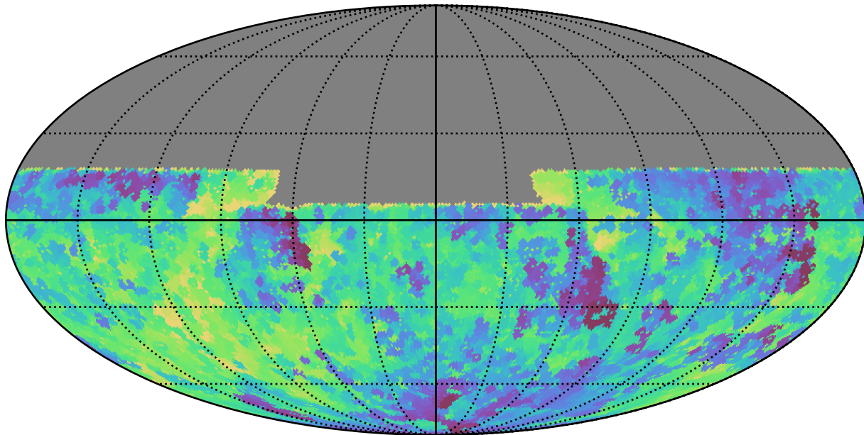
baseline_v2.0_10yrs All sky u band: Min fiveSigmaDepth
