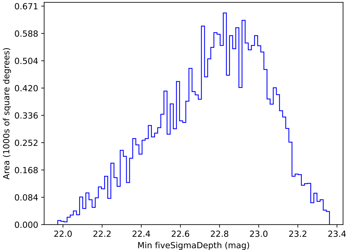
baseline_v2.0_10yrs All sky u band: Min fiveSigmaDepth
