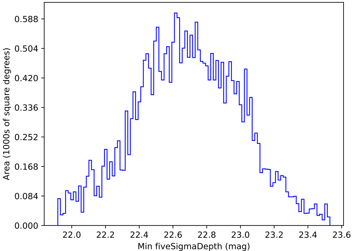
baseline_v2.0_10yrs All sky r band: Min fiveSigmaDepth
