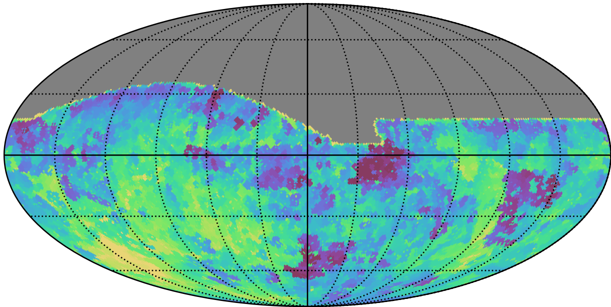
baseline_v2.0_10yrs All sky i band: Min fiveSigmaDepth
