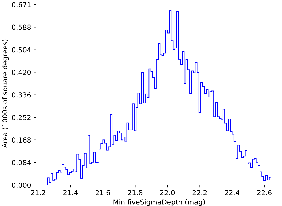
baseline_v2.0_10yrs All sky i band: Min fiveSigmaDepth
