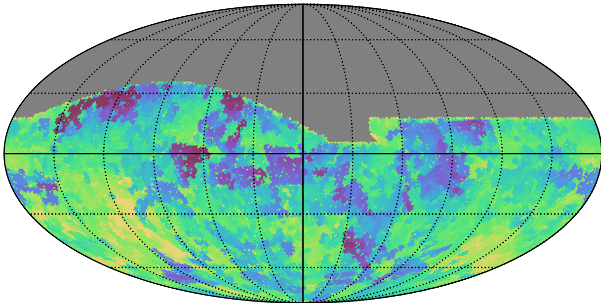
baseline_v2.0_10yrs All sky g band: Min fiveSigmaDepth
