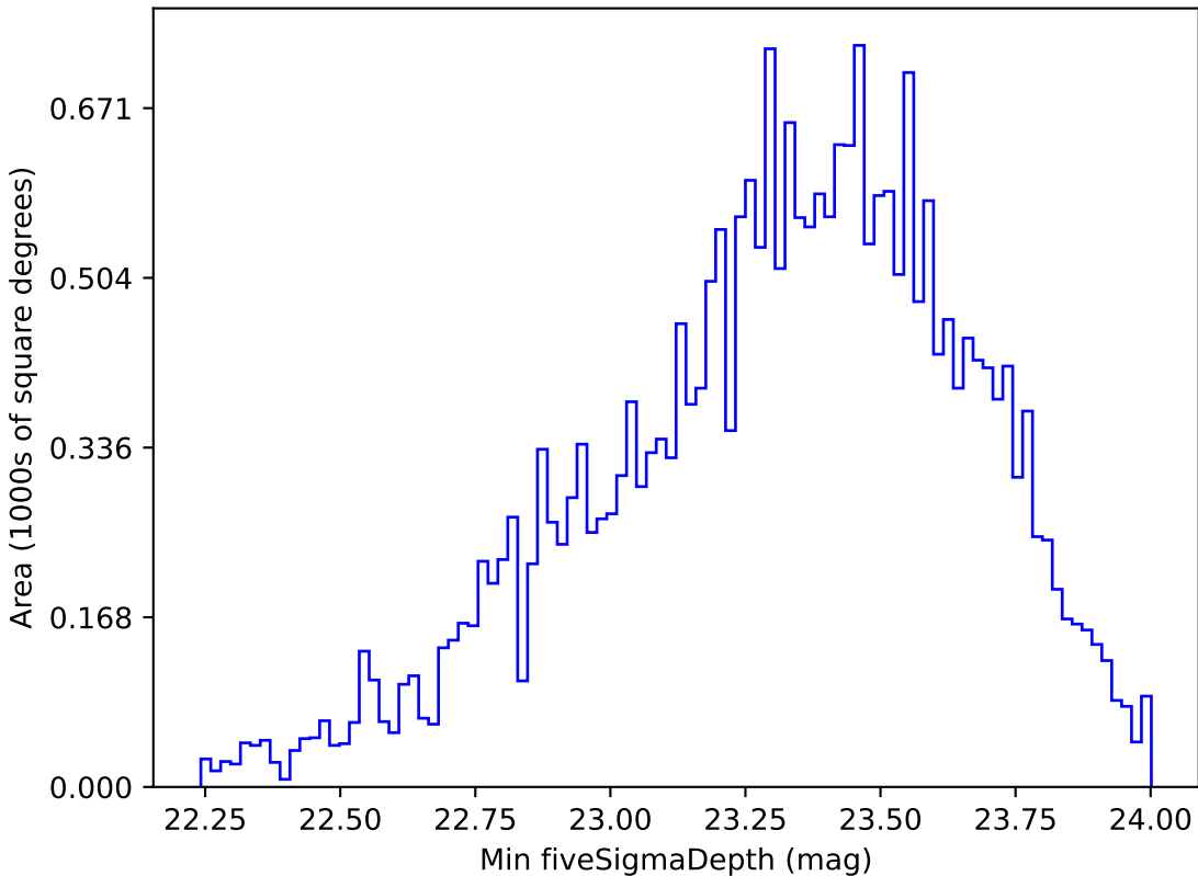
baseline_v2.0_10yrs All sky g band: Min fiveSigmaDepth
