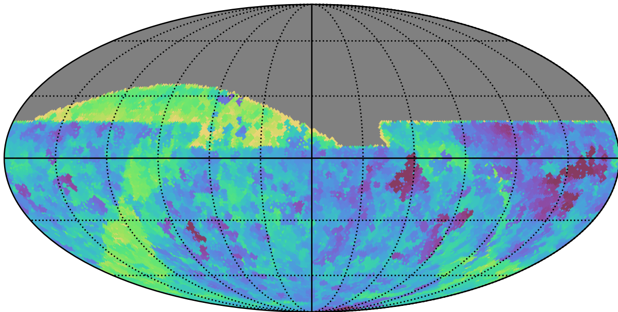
baseline_v2.0_10yrs All sky all bands: Min fiveSigmaDepth
