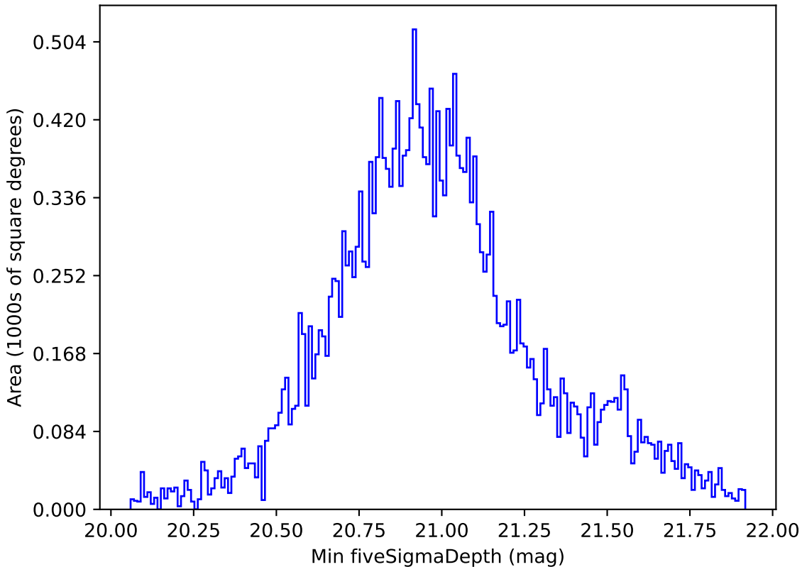
baseline_v2.0_10yrs All sky all bands: Min fiveSigmaDepth
