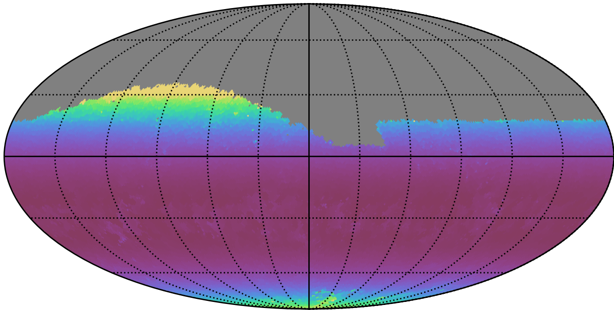
baseline_v2.0_10yrs Yr 1 z band: Min airmass
