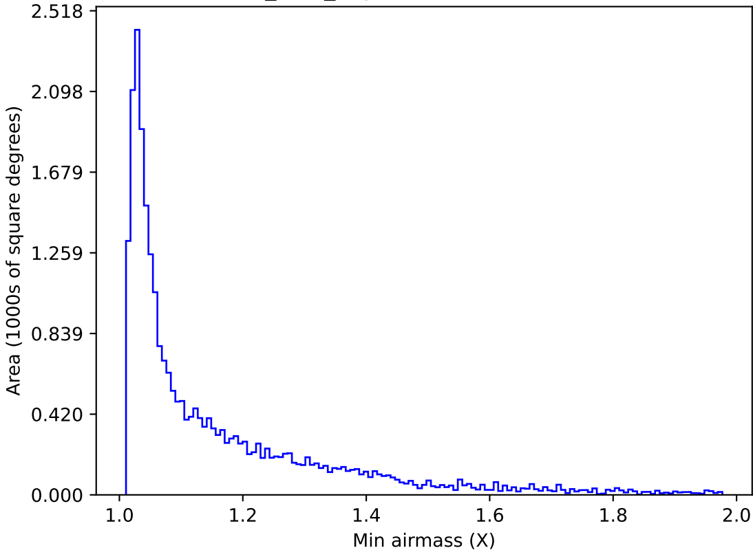
baseline_v2.0_10yrs Yr 1 z band: Min airmass
