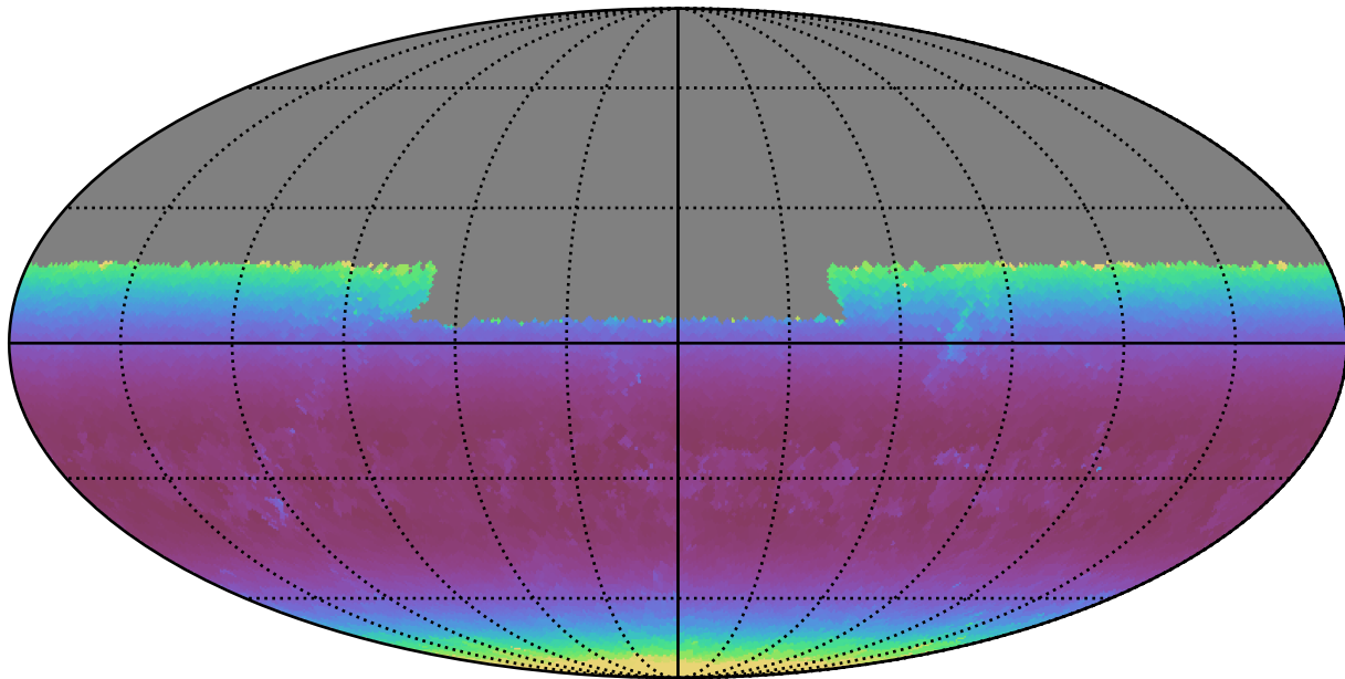
baseline_v2.0_10yrs Yr 1 y band: Min airmass
