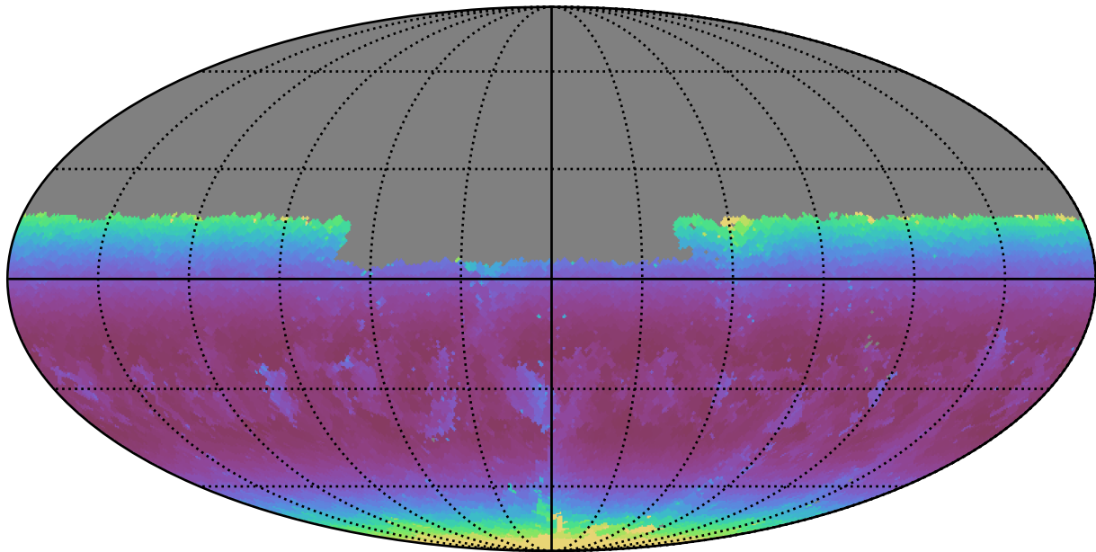
baseline_v2.0_10yrs Yr 1 u band: Min airmass
