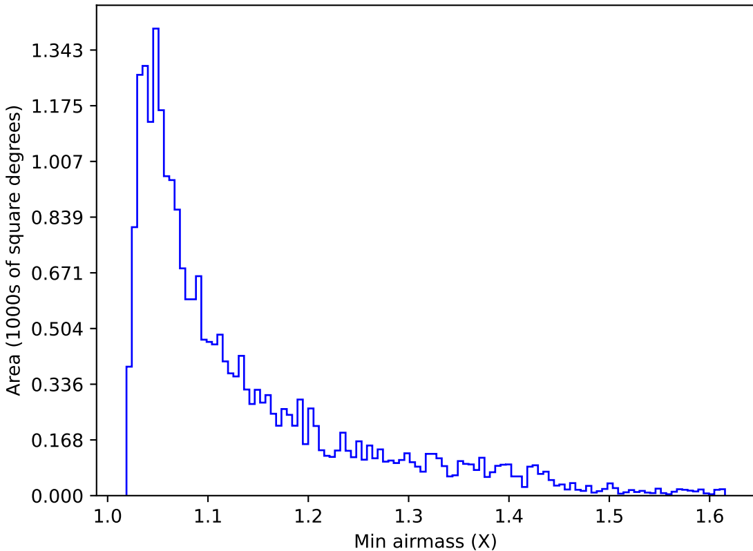
baseline_v2.0_10yrs Yr 1 u band: Min airmass
