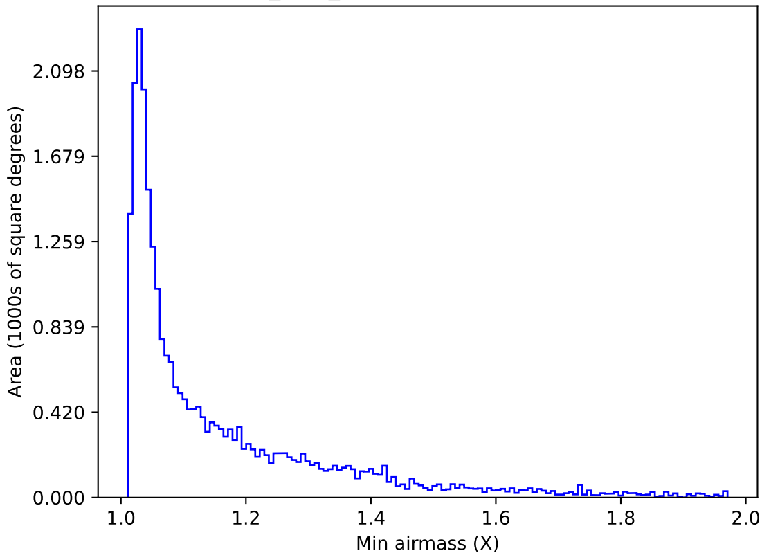
baseline_v2.0_10yrs Yr 1 r band: Min airmass
