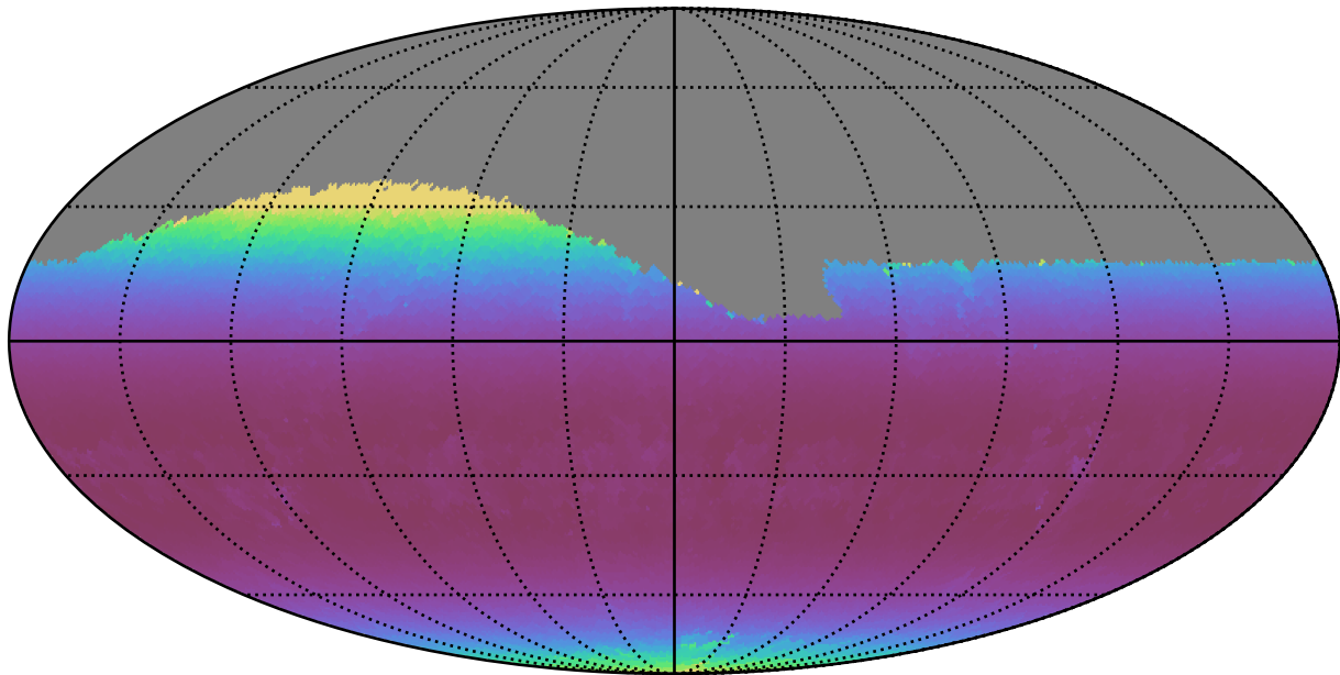
baseline_v2.0_10yrs Yr 1 i band: Min airmass
