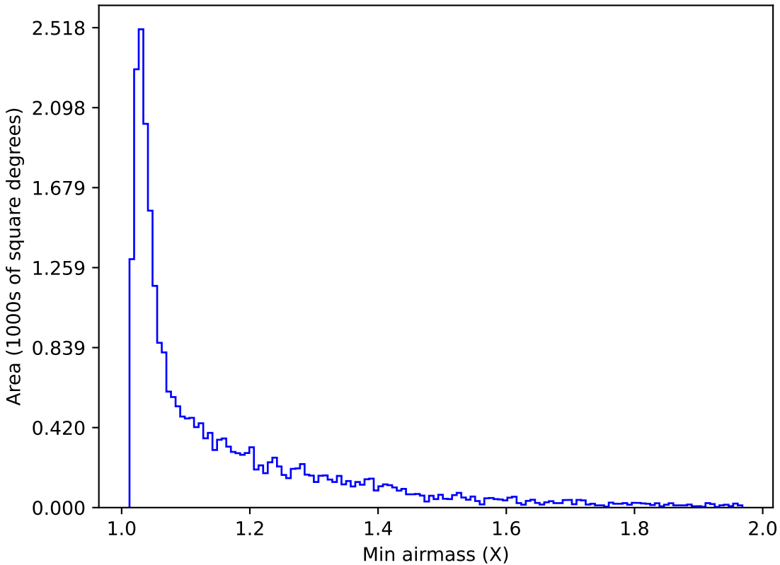
baseline_v2.0_10yrs Yr 1 i band: Min airmass
