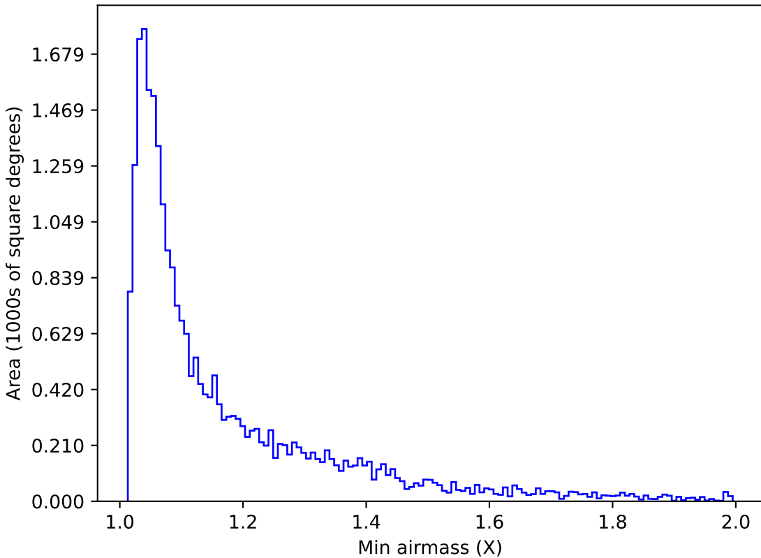
baseline_v2.0_10yrs Yr 1 g band: Min airmass
