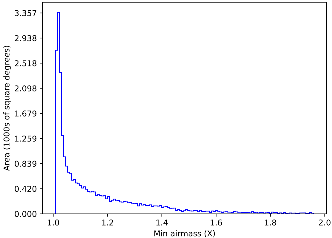
baseline_v2.0_10yrs Yr 1 all bands: Min airmass
