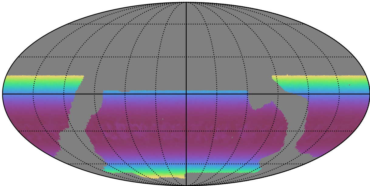
baseline_v2.0_10yrs WFD z band: Min airmass
