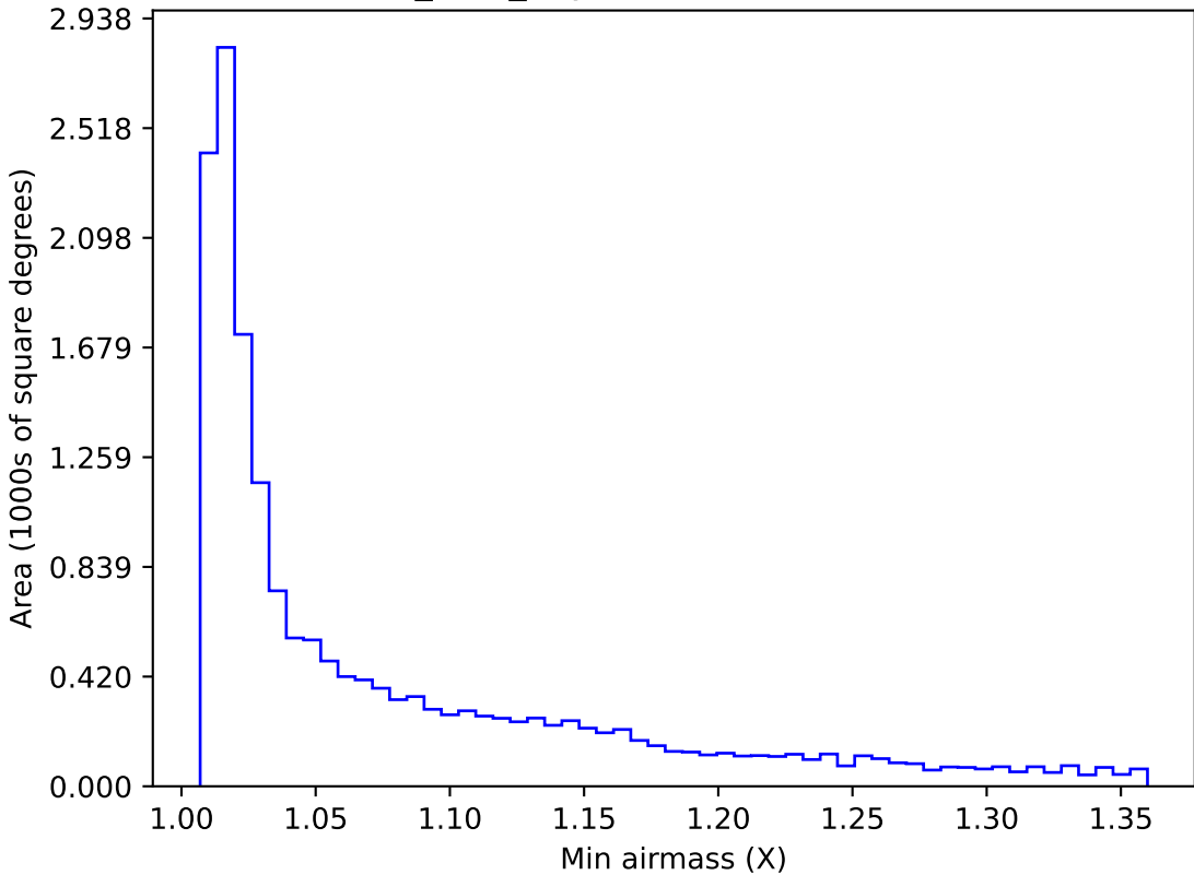
baseline_v2.0_10yrs WFD z band: Min airmass
