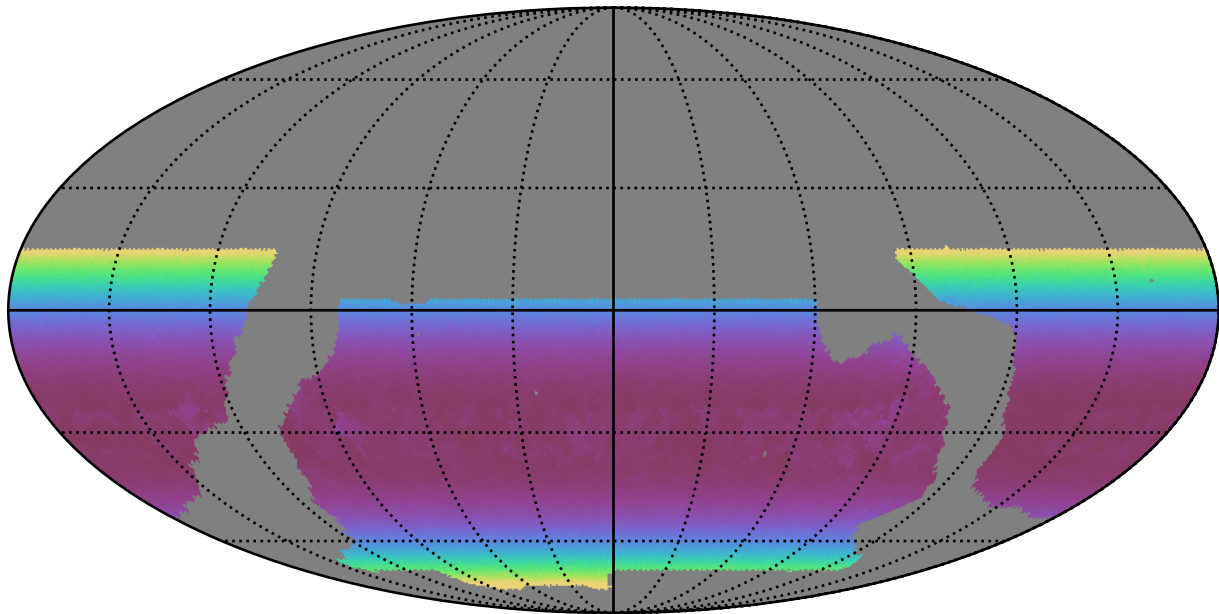
baseline_v2.0_10yrs WFD y band: Min airmass
