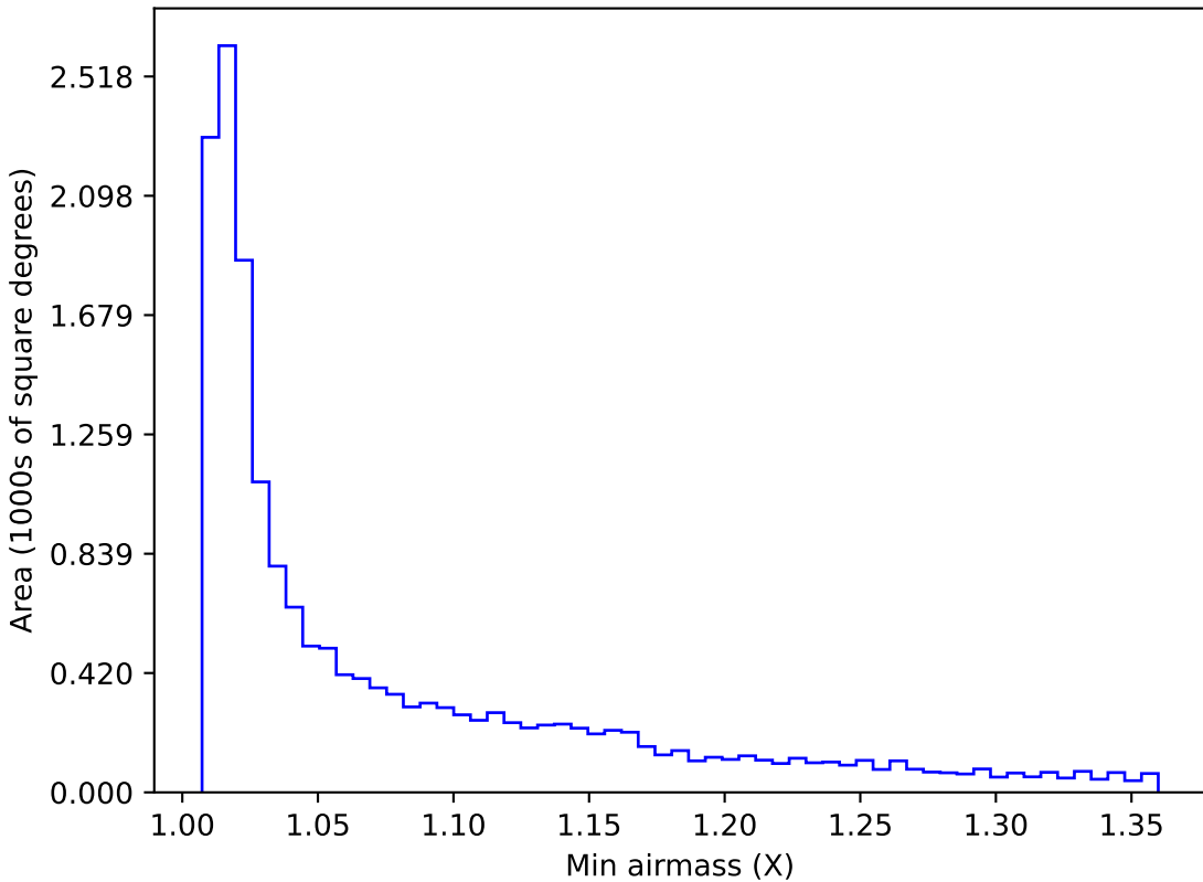
baseline_v2.0_10yrs WFD y band: Min airmass
