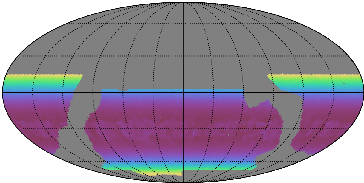
baseline_v2.0_10yrs WFD u band: Min airmass
