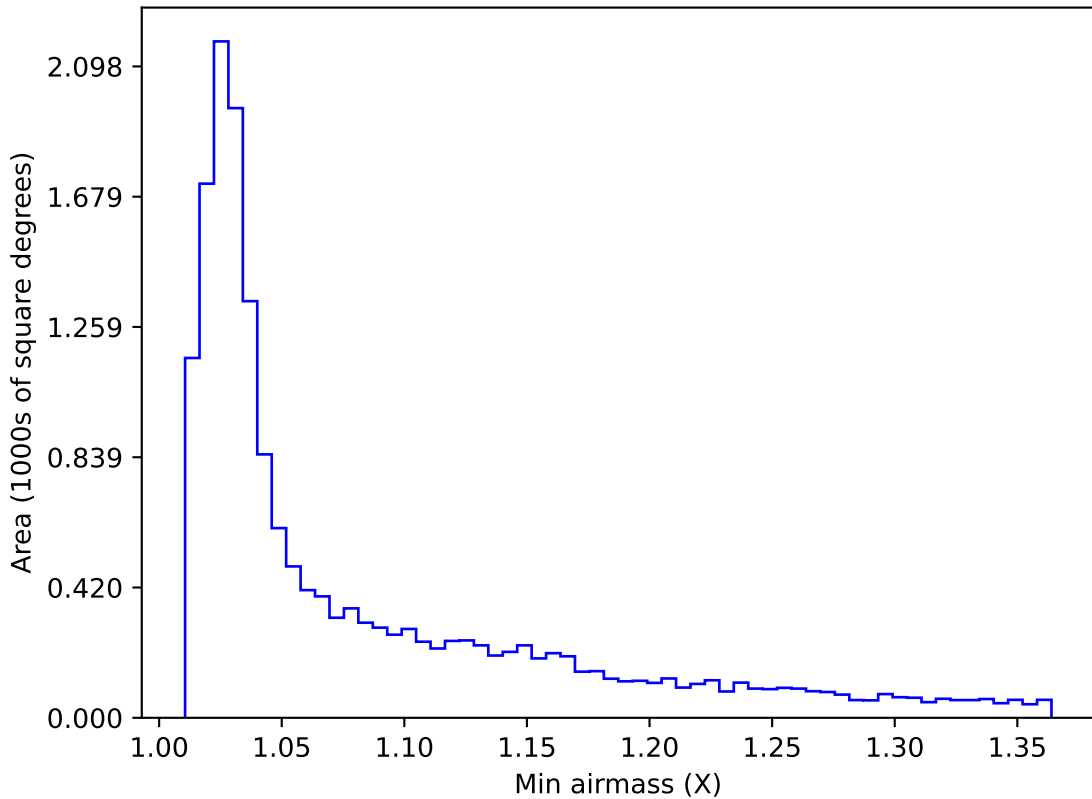
baseline_v2.0_10yrs WFD u band: Min airmass
