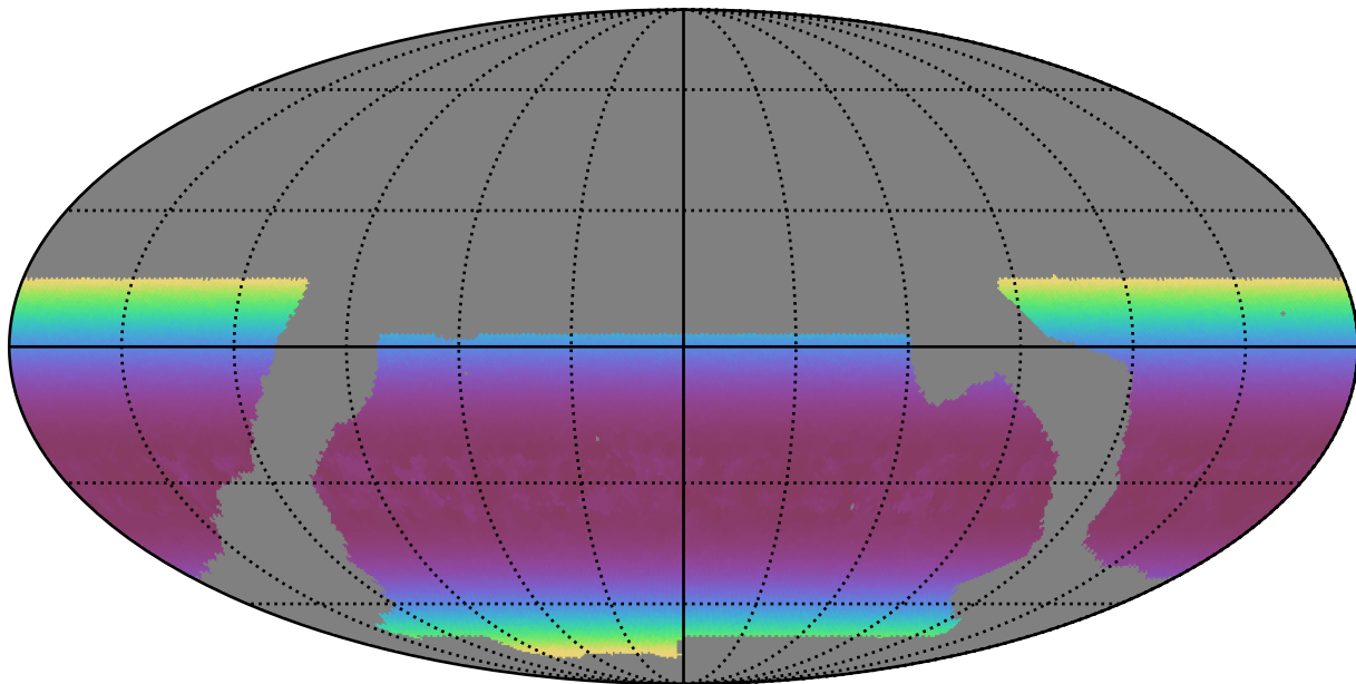
baseline_v2.0_10yrs WFD r band: Min airmass
