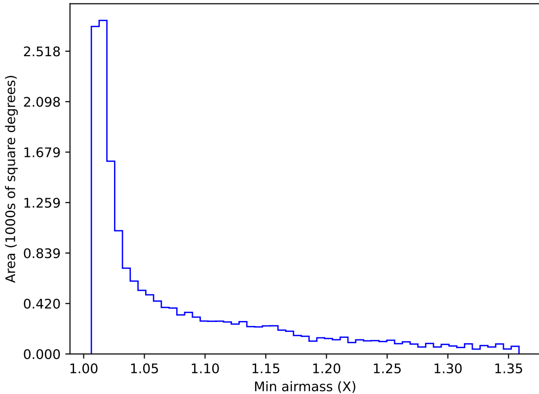
baseline_v2.0_10yrs WFD r band: Min airmass
