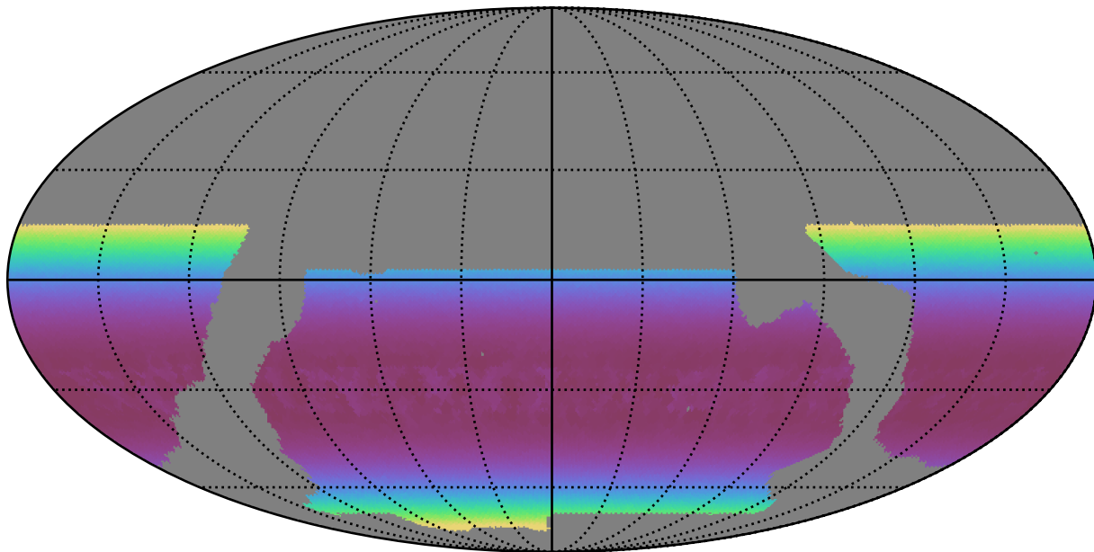
baseline_v2.0_10yrs WFD i band: Min airmass
