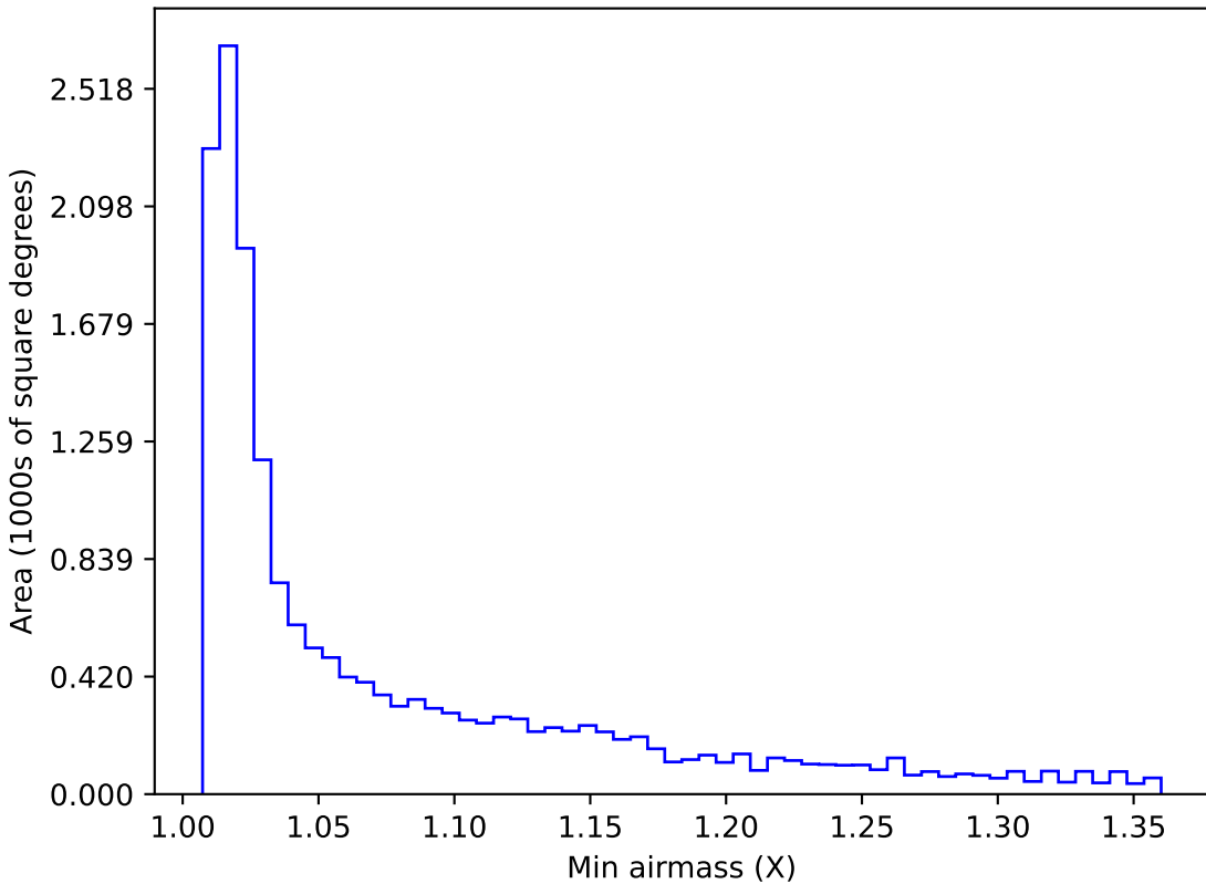
baseline_v2.0_10yrs WFD i band: Min airmass
