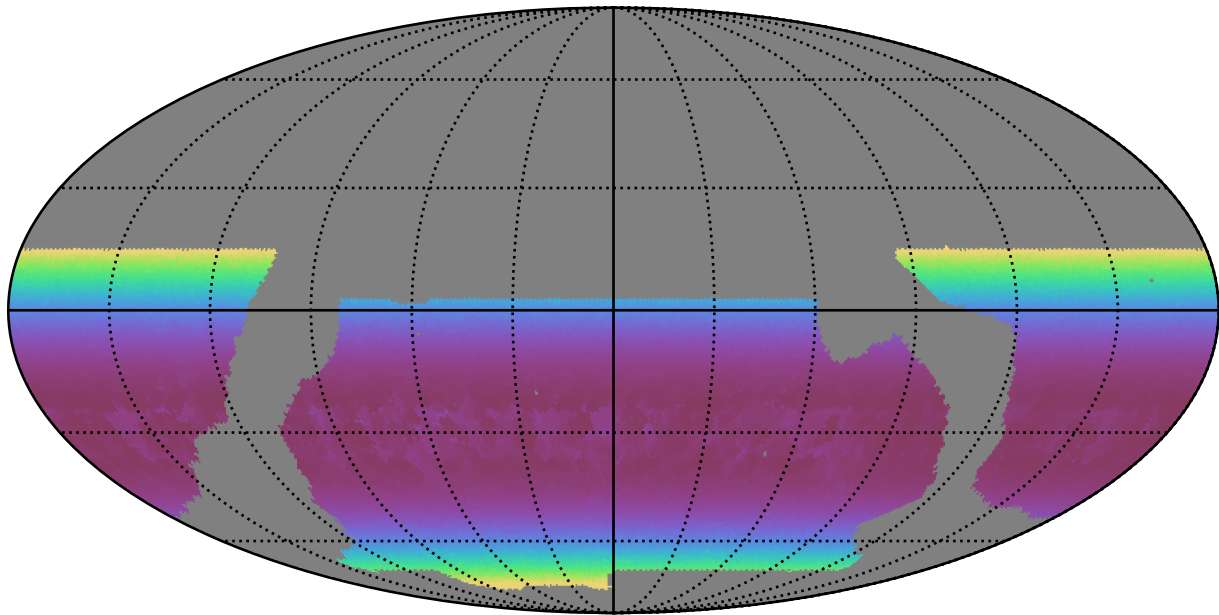
baseline_v2.0_10yrs WFD g band: Min airmass
