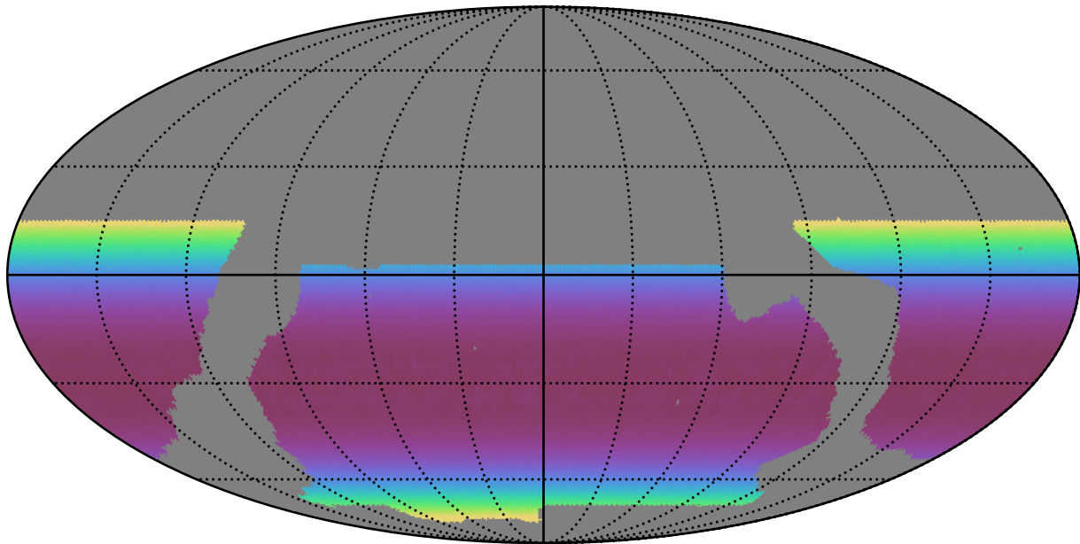
baseline_v2.0_10yrs WFD all bands: Min airmass
