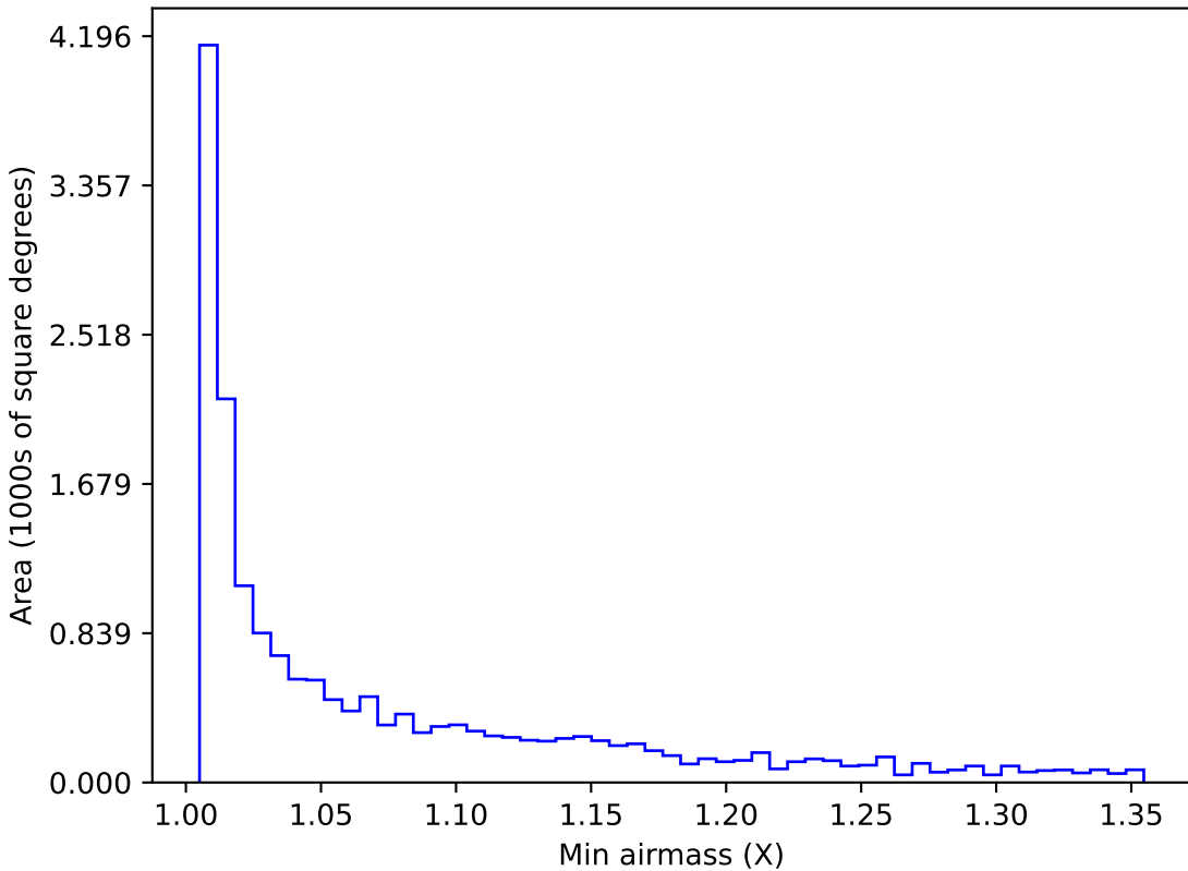
baseline_v2.0_10yrs WFD all bands: Min airmass
