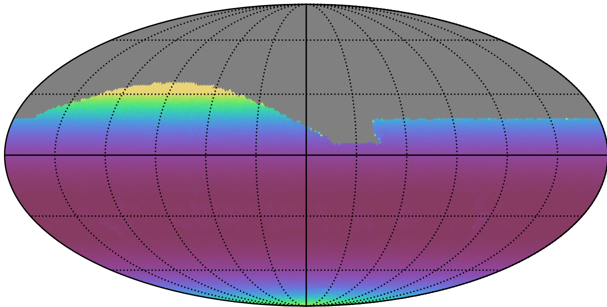
baseline_v2.0_10yrs All sky z band: Min airmass
