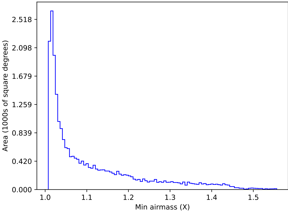
baseline_v2.0_10yrs All sky y band: Min airmass
