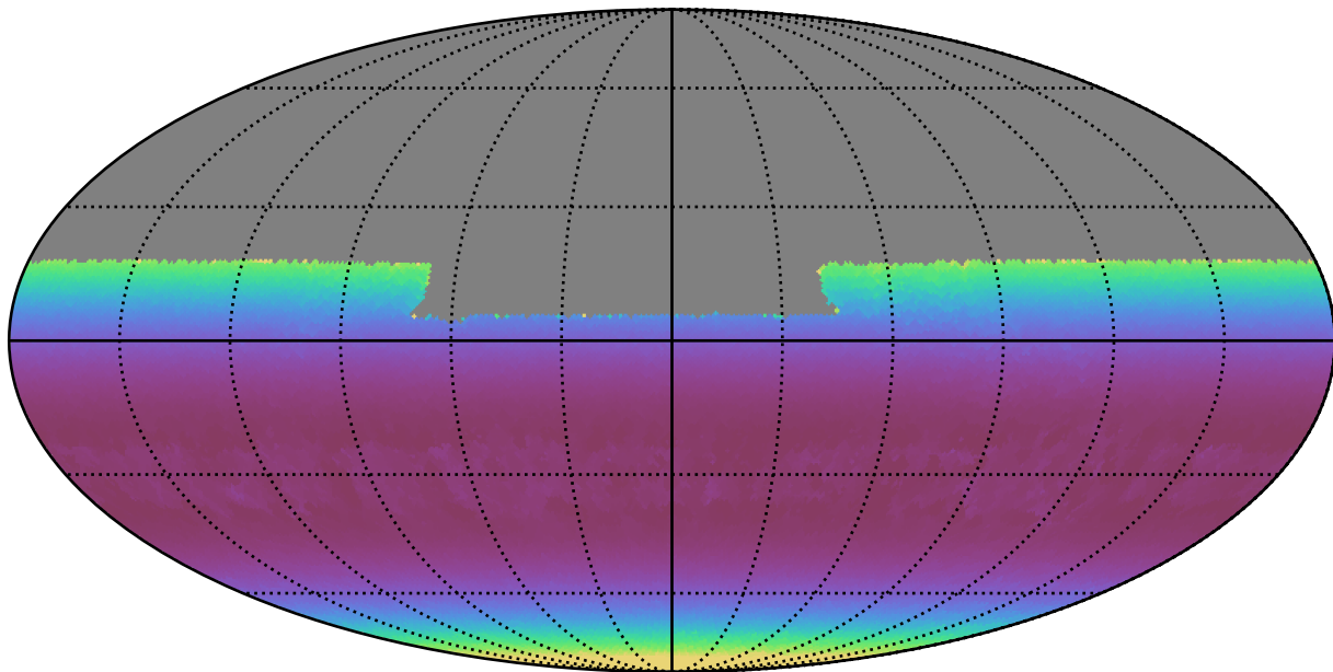
baseline_v2.0_10yrs All sky u band: Min airmass
