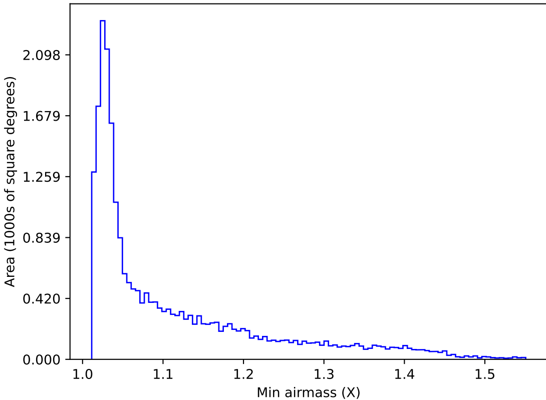
baseline_v2.0_10yrs All sky u band: Min airmass
