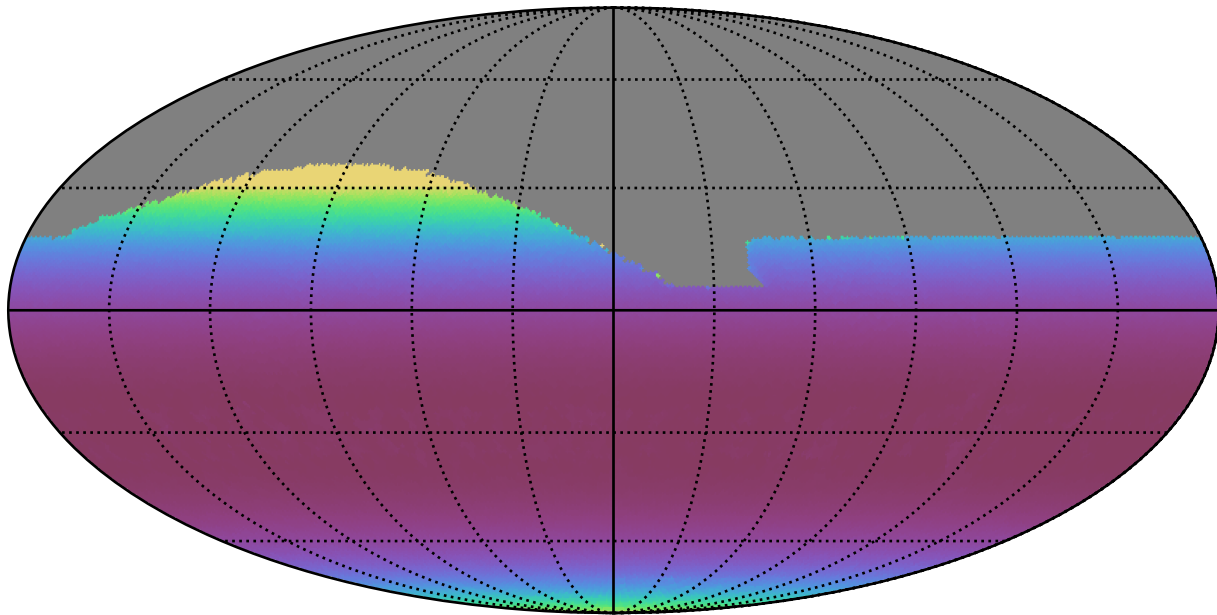
baseline_v2.0_10yrs All sky r band: Min airmass
