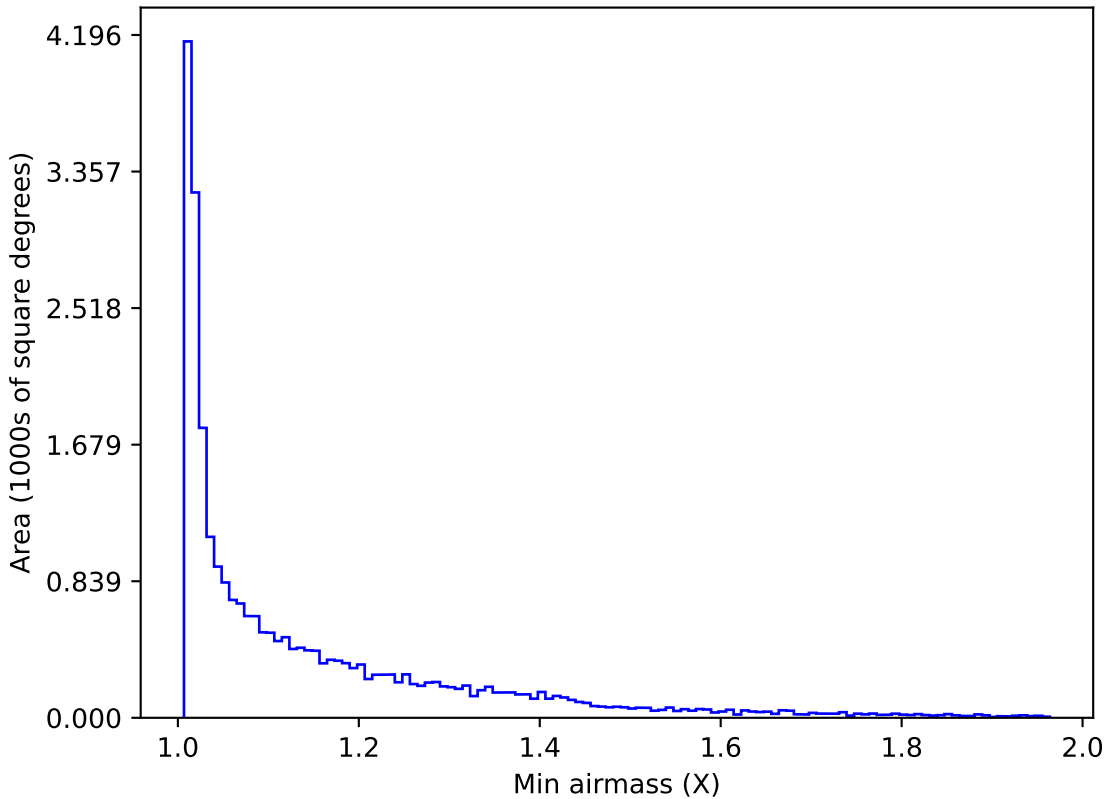
baseline_v2.0_10yrs All sky r band: Min airmass
