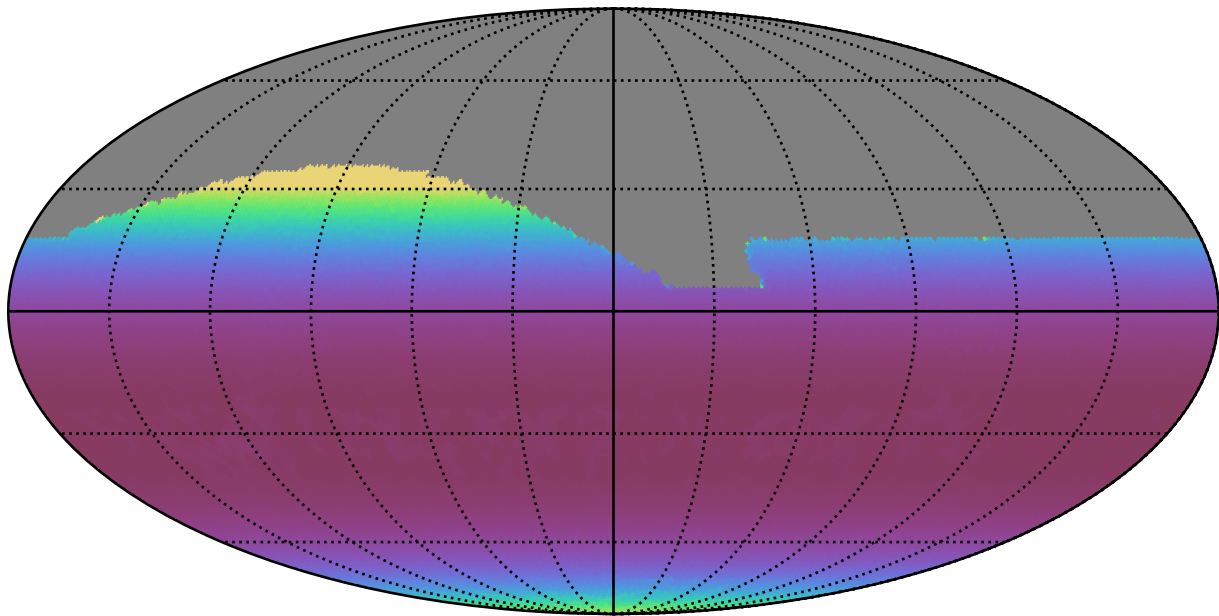
baseline_v2.0_10yrs All sky i band: Min airmass
