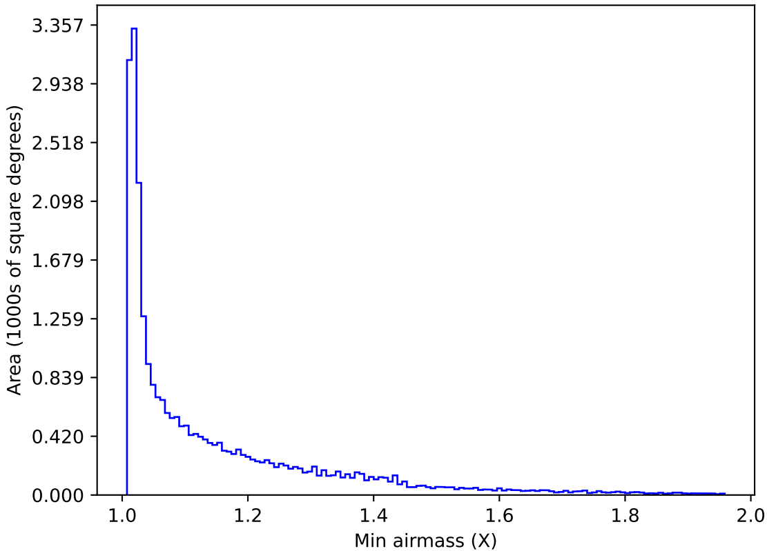
baseline_v2.0_10yrs All sky i band: Min airmass
