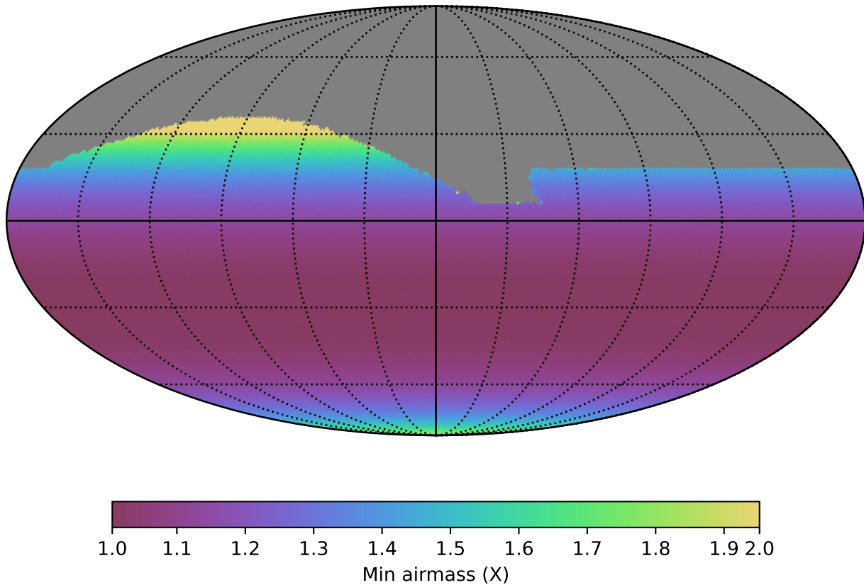
baseline_v2.0_10yrs All sky all bands: Min airmass
