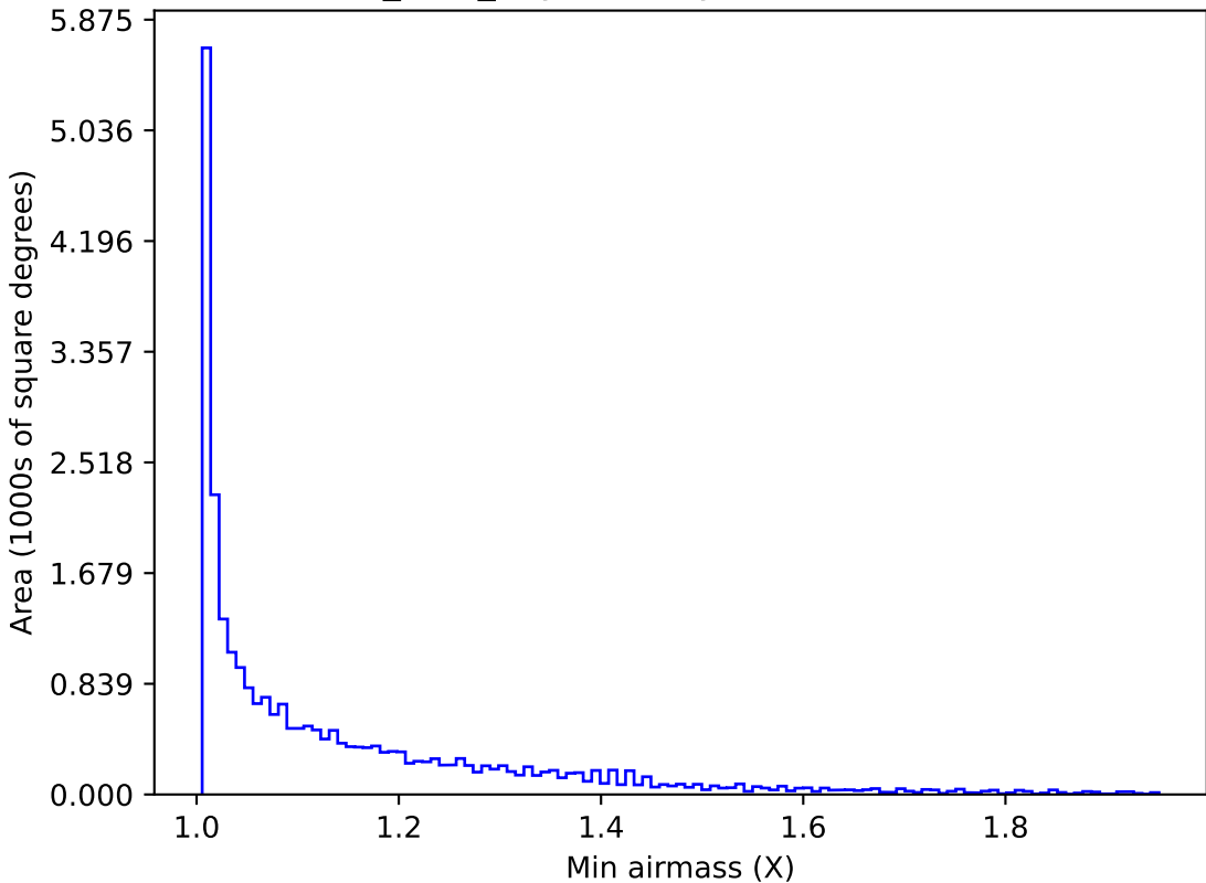
baseline_v2.0_10yrs All sky all bands: Min airmass
