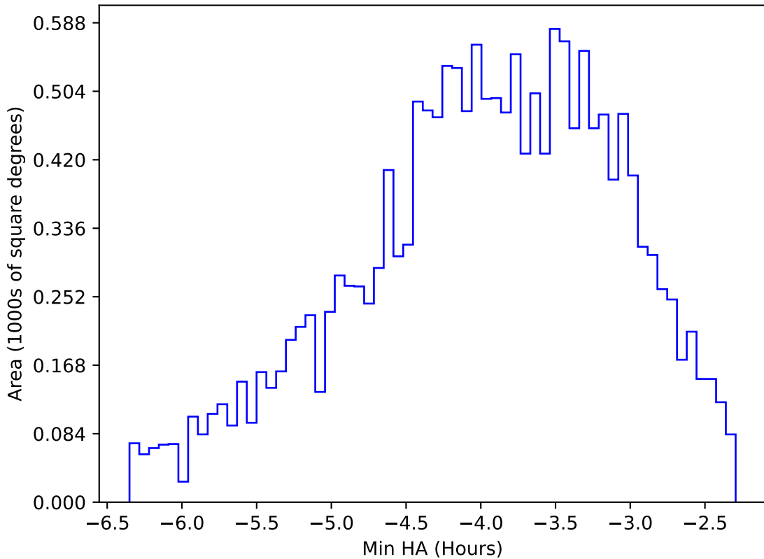
baseline_v2.0_10yrs WFD all bands: Min HA
