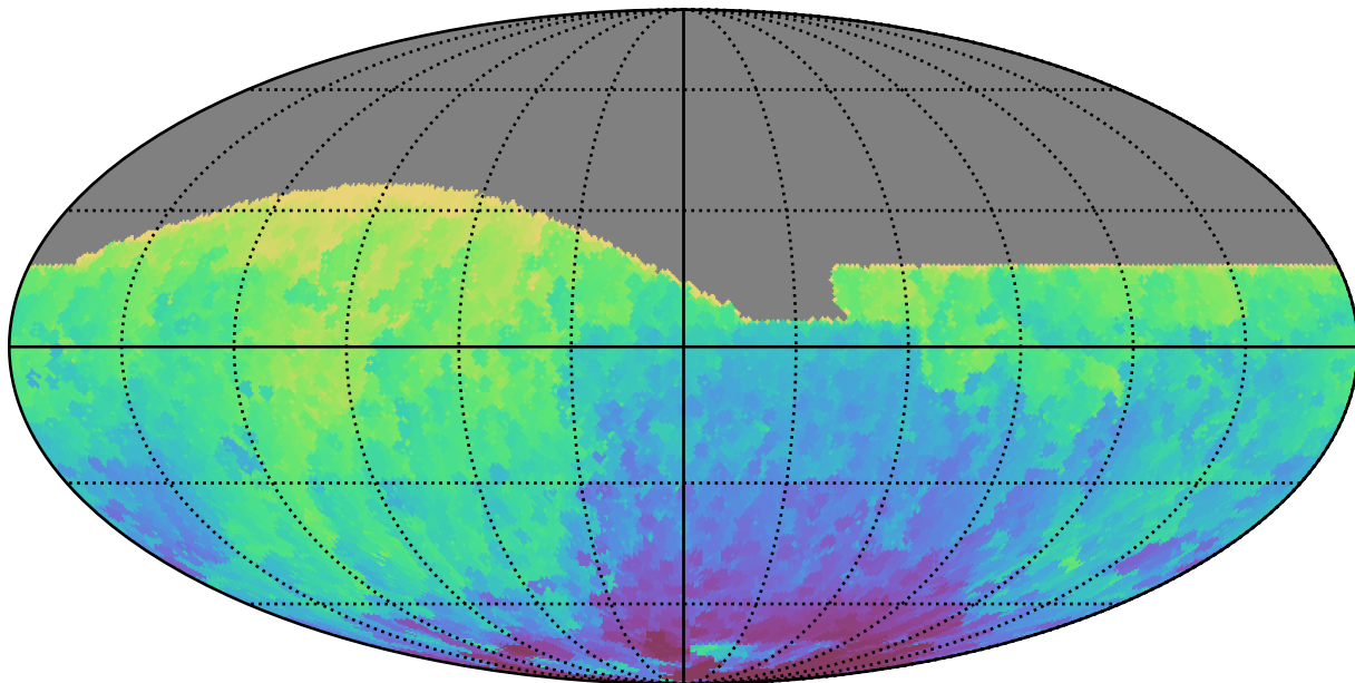
baseline_v2.0_10yrs All sky all bands: Min HA
