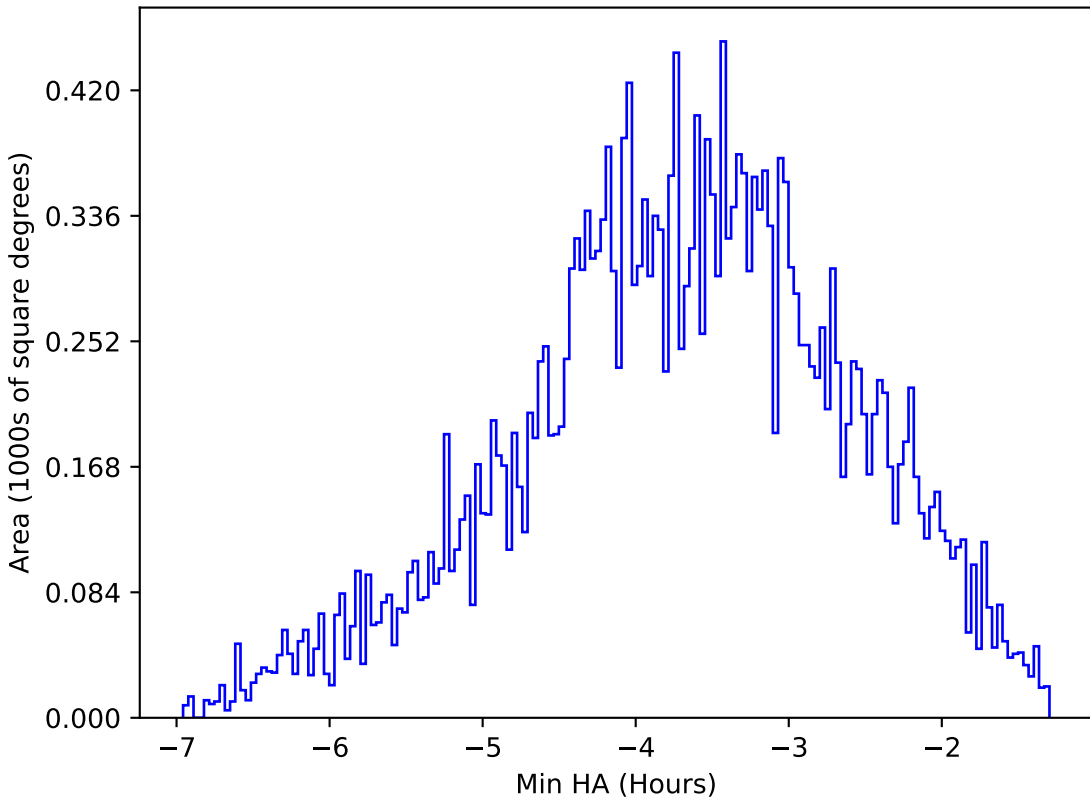
baseline_v2.0_10yrs All sky all bands: Min HA
