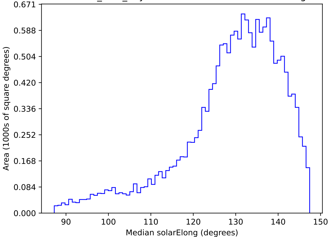
baseline_v2.0_10yrs WFD z band: Median solarElong
