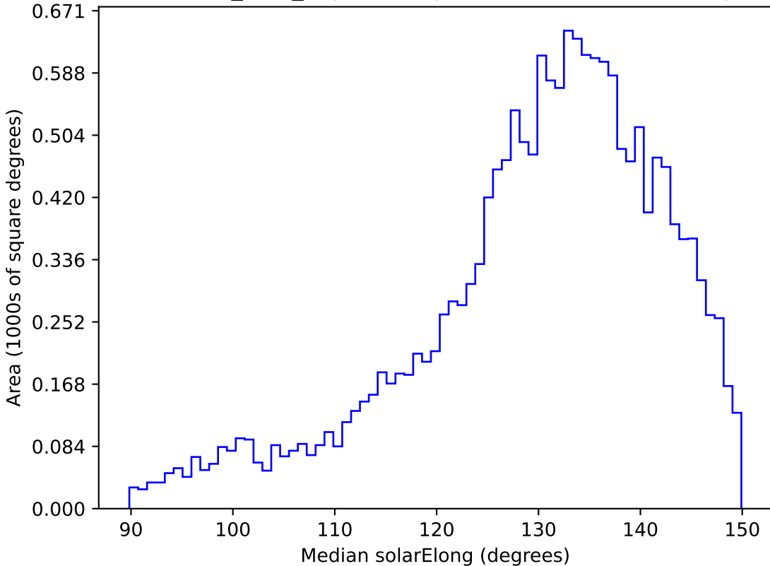
baseline_v2.0_10yrs WFD y band: Median solarElong
