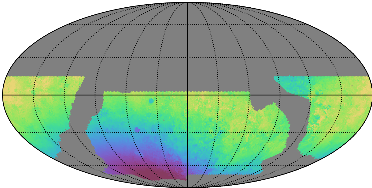
baseline_v2.0_10yrs WFD u band: Median solarElong
